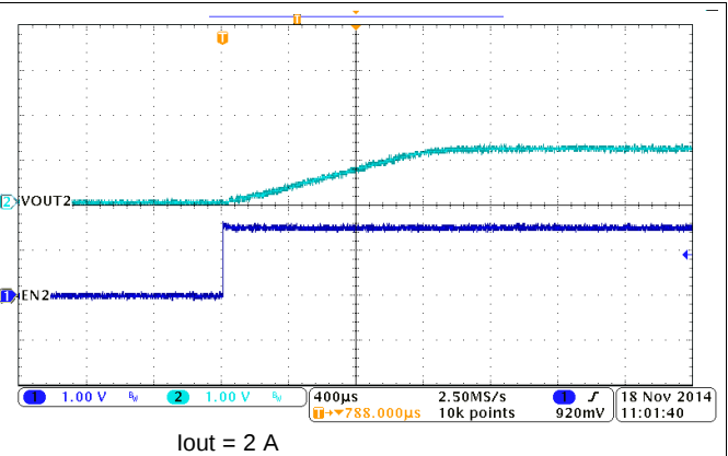
Figure 45. BUCK2, Soft-Start
