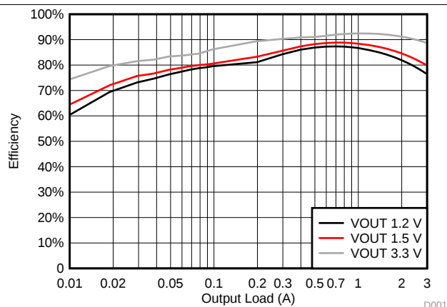
Figure 1. BUCK1 Efficiency
