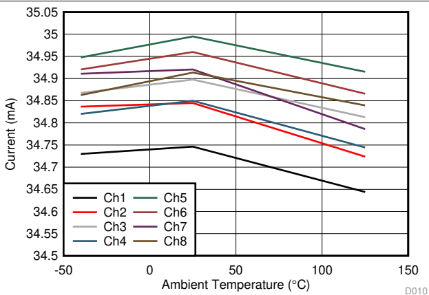
Figure 4. I_{(IOUTX)} Accuracy vs Ambient Temperature
