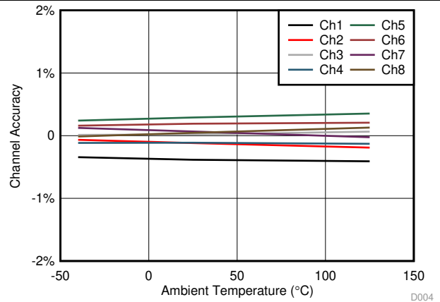
Figure 2. I_{(IOUTX)} Accuracy vs Ambient Temperature
