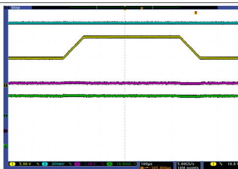
CH1: V_{(SUPPLY)} CH2: V_{(REF)} CH3: V_{(FAULT)} CH4: I_{(OUT8)} I_{(OUTx)} = 35 mA
