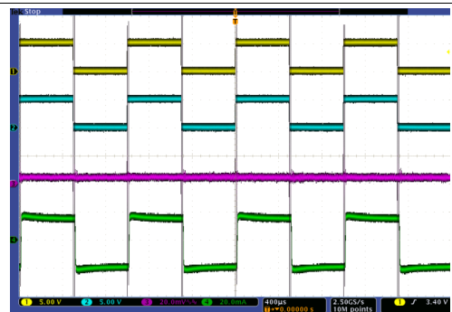
CH1: V_{(PWM3)} CH2: V_{(PWM4)} CH3: V_{(REF)} CH4: I_{(OUT8)} Duty cycle = 50% V_{(SUPPLY)} , V_{(EN)} = 14 V
