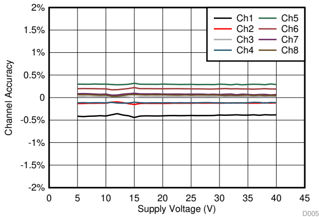
Figure 1. I_{(IOUTX)} Accuracy vs V_{(SUPPLY)}
