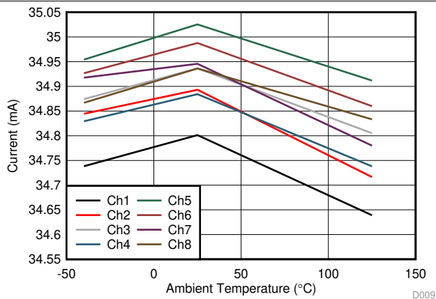
Figure 3. I_{(IOUTX)} Accuracy vs Ambient Temperature
