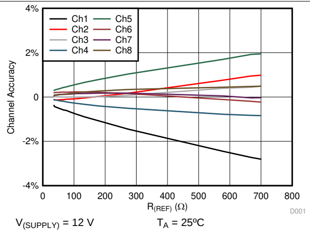
Figure 8. I_{(IOUTx)} Channel Accuracy vs R_{(REF)}
