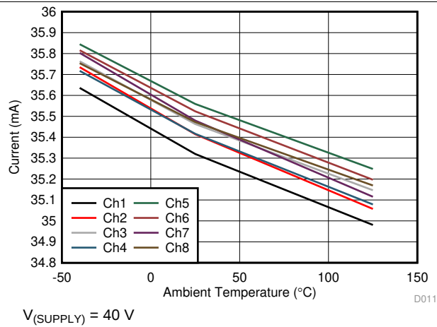
Figure 7. I_{(IOUTx)} Current vs Temperature
