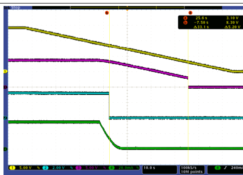
CH1: V_{(SUPPLY)} CH2: V_{(FAULT)} CH3: V_{(REF)} CH4: I_{(OUT8)}
