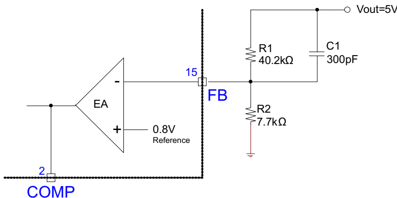
Figure 35. Buck Feedback Resistor Divider
