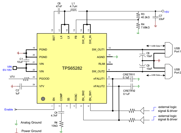
Figure 41. Auto Retry Functionality With External Enable Signal
