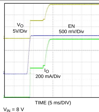
Figure 12. Start-Up Waveforms
