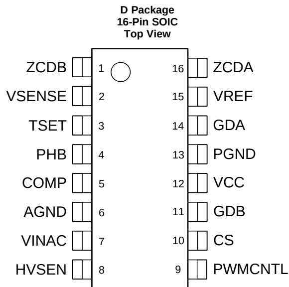
Pin Functions
