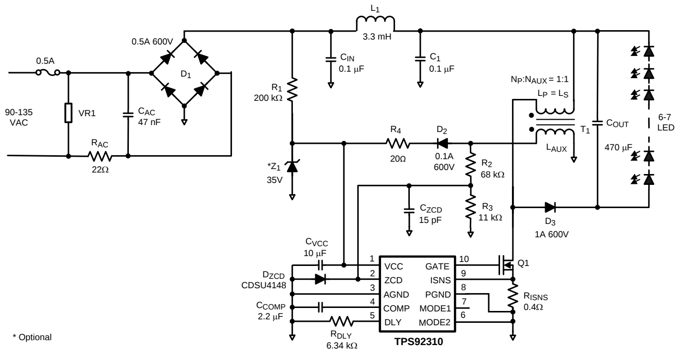
Figure 26. Non-isolated topology schematic
