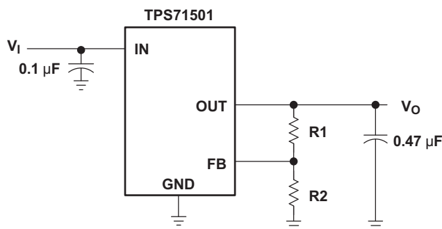
Figure 15. TPS71501 Adjustable LDO Regulator Programming
