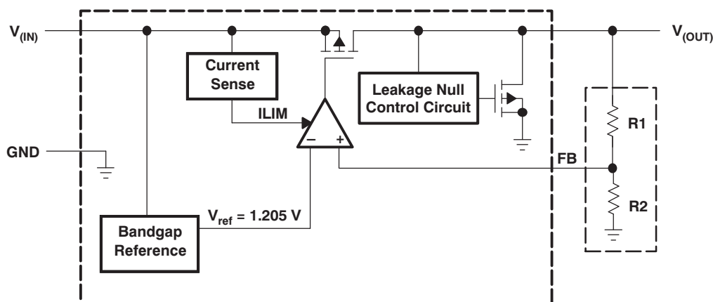
Figure 13. Functional Block Diagram—Adjustable Version
