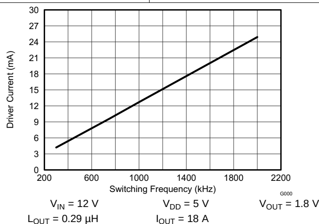
Figure 9. Driver Current vs Frequency
