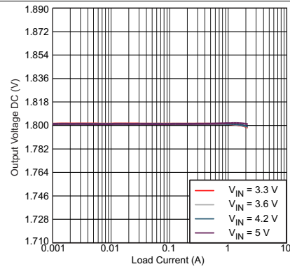
Figure 15. Output Voltage Accuracy vs Load Current Forced PWM MODE
