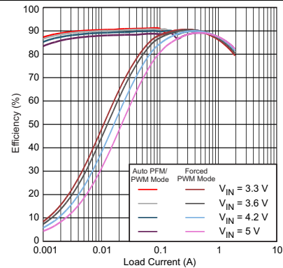
Figure 11. Efficiency vs Load Current PFM and PWM MODE
