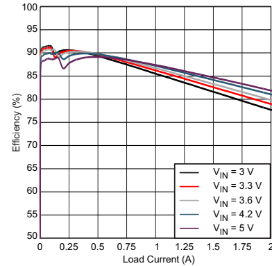
Figure 11. Efficiency vs Load Current PFM and PWM MODE
