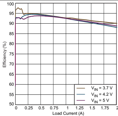
Figure 10. Efficiency vs Load Current Auto PFM and PWM MODE
