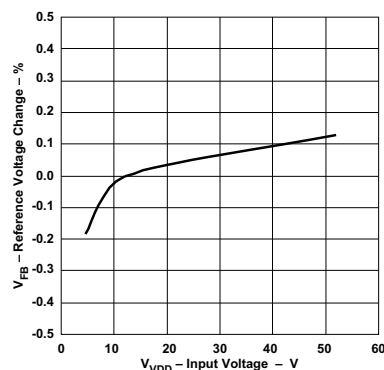
Figure 6. Reference Voltage Change vs Input Voltage
