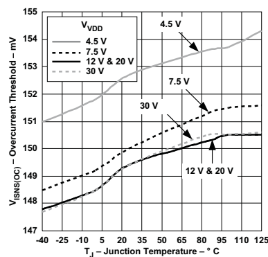
Figure 8. Overcurrent Threshold vs Junction Temperature
