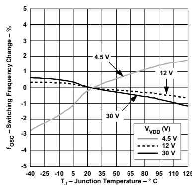
Figure 10. Switching Frequency Change vs Junction Temperature
