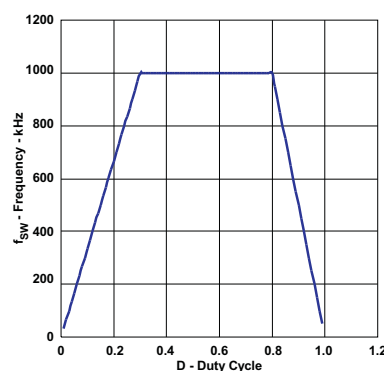
Figure 2. Switching Frequency vs Duty Cycle
