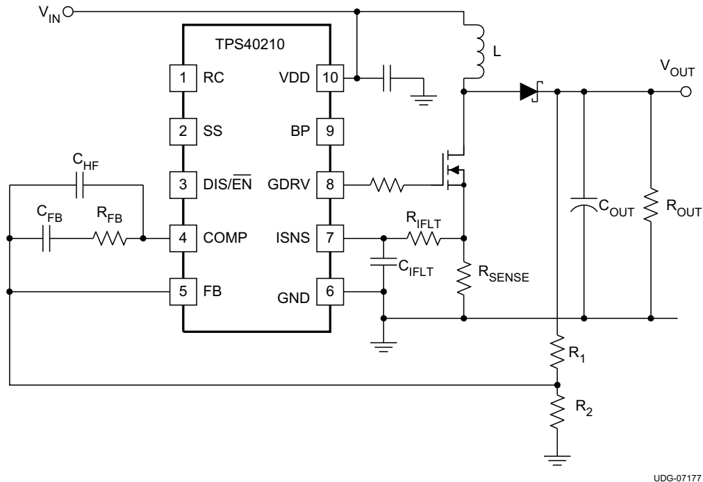
Figure 27. Basic Compensation Network
