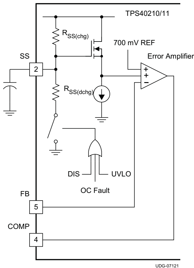
Figure 21. SS Pin Functional Circuit
