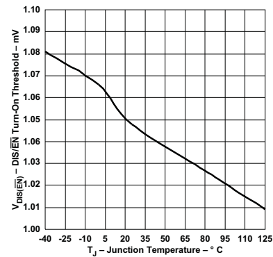
Figure 18. DIS/EN Turn-On Threshold vs Junction Temperature
