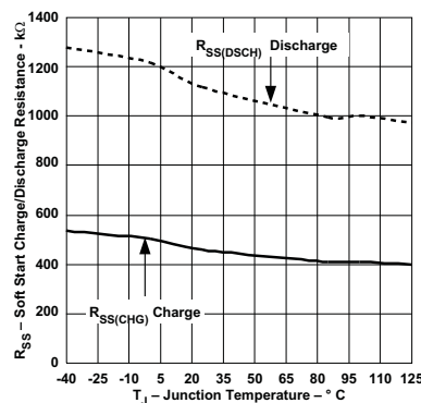
Figure 12. Soft Start Charge/Discharge Resistance vs Junction Temperature
