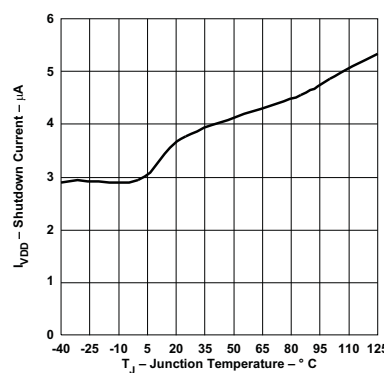
Figure 4. Shutdown Current vs Junction Temperature
