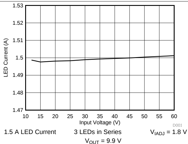
Figure 2. Line Regulation
