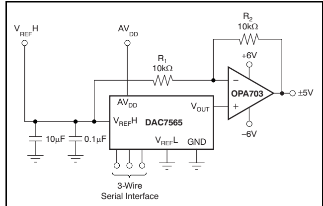
Figure 99. Bipolar Output Range Using External Reference at 5V
