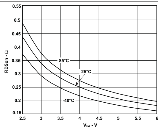
Figure 4. R_{DSon} PMOS vs V_{IN}
