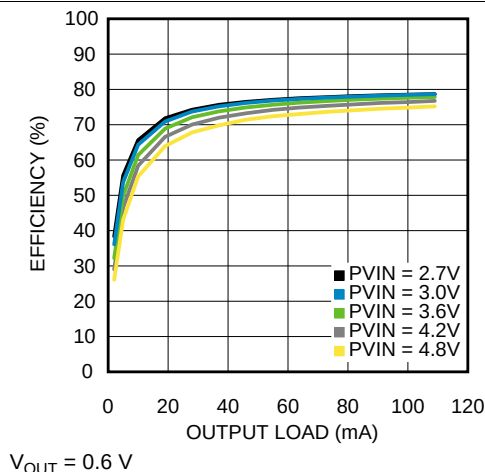
Figure 4. PFM Efficiency
