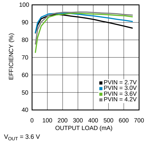
Figure 8. PWM Efficiency
