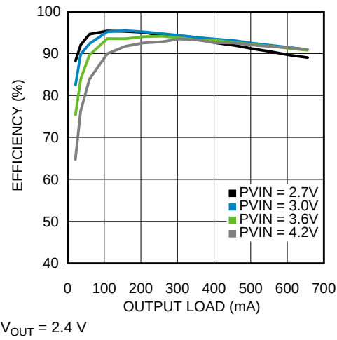
Figure 7. PWM Efficiency
