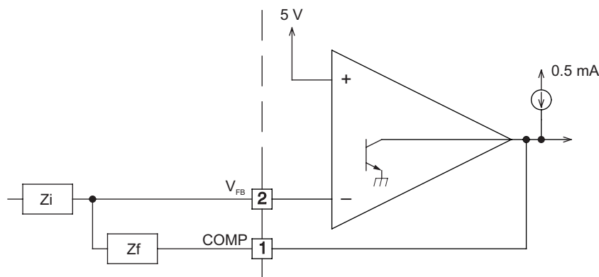
Figure 19. E/A Configuration
