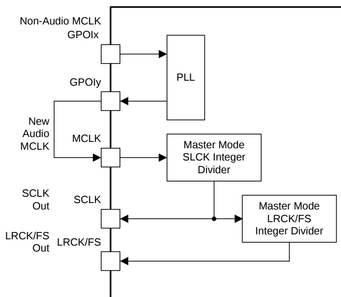
Figure 63. Generating Audio Clocks Using Non-Audio Clock Sources
