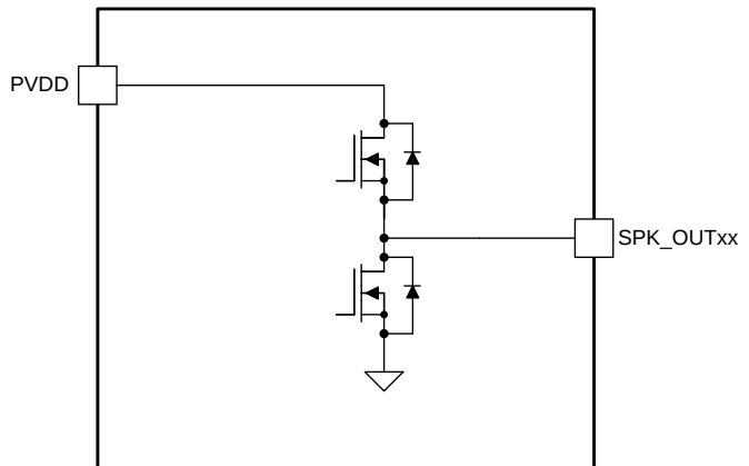
Figure 4. SPK_OUTxx Pins
